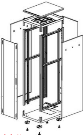
Explode View
